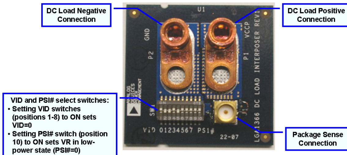
Figure 1. VR11.1 DC Load Interposer
